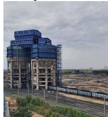
Silo Facility with telscopic chute system
